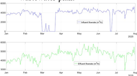
Fig. 1. Wastewater throughput at Someșeni
